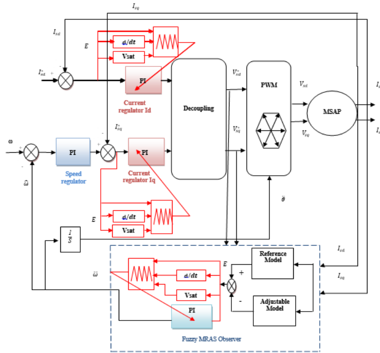
Figure 5. Block diagram of sensorless vector control of PMSM
