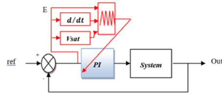
Figure 2. Block diagram of the proposed control system.
