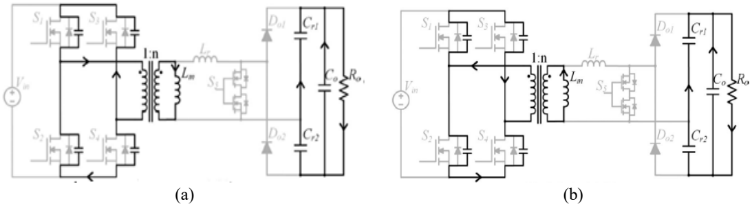
Figure 5. Operation modes; (a) mode 4, and (b) mode 8
