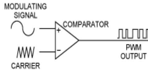
Figure 4. A comparator configuration to produce a PWM signal
