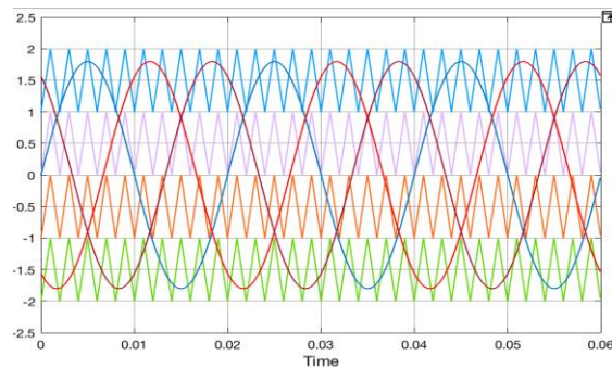
Figure 7. Carrier arrangement for MCPWM strategy of three phase five-level inverter
