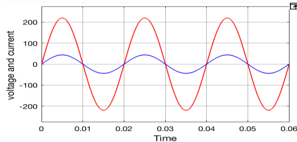
Figure 13. Output current and voltage of grid connected inverter supplied a linear load
