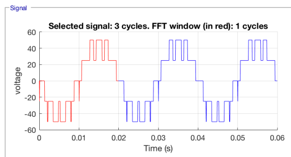
Figure 3. Five-level inverter waveform
