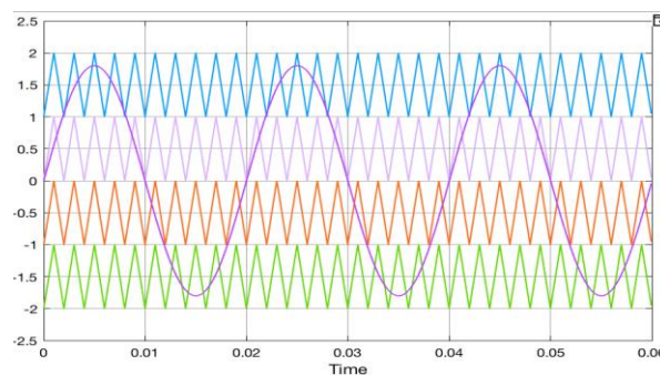
Figure 5. Carrier arrangement for MCPWM strategy of single five-level inverters
