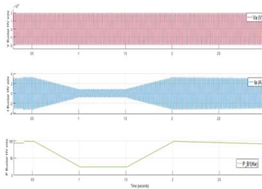
Figure 9. Simulated Voltage, Current and Power at transfomer HV side using the P&O MPPT Algorithm
