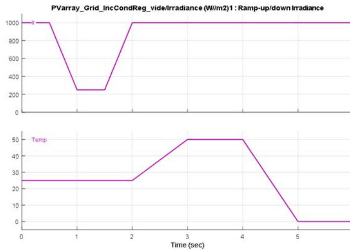
Figure 7. Simulated weather conditions (Irradiance and Temperature levels)
