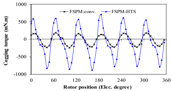
Figure 7. Cogging torque
