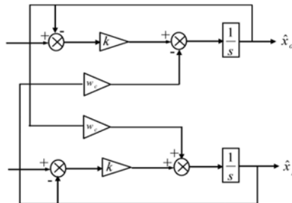
Figure 1. Self-tuning filter
