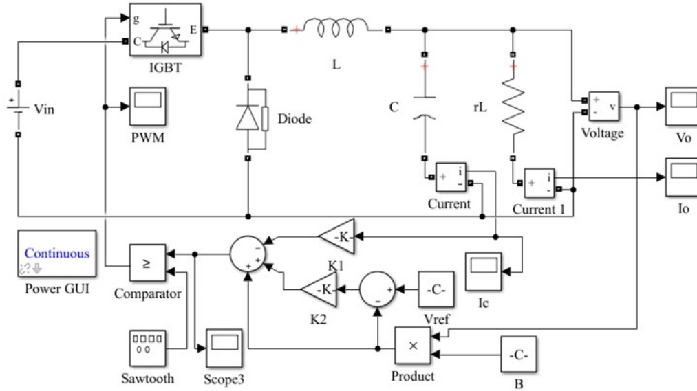
Figure 6. Modeling of DC/DC buck converter based on SMC using matlab /simulink
