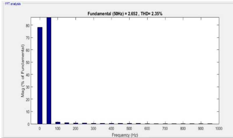
Figure 5. THD output voltage for 5-level cascaded h-bridge mvsii (filter)
