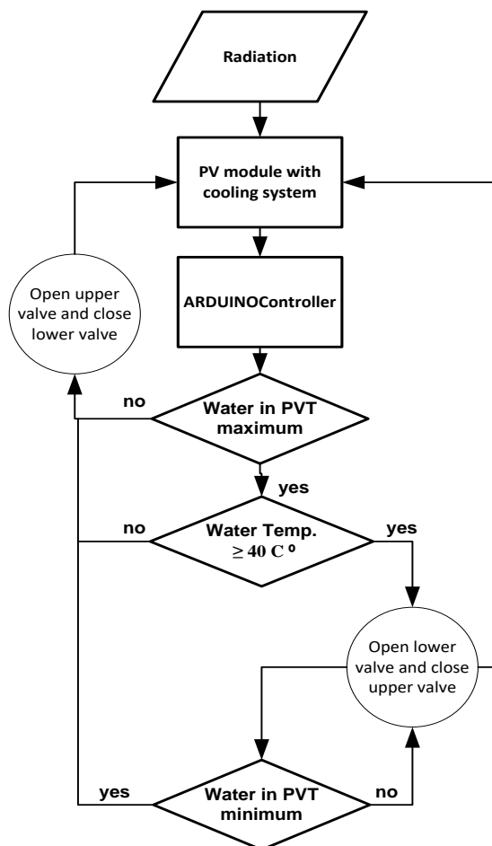
Figure 5. Flowchart of the PV-T system process
