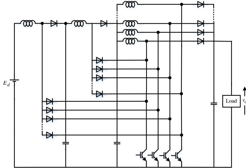
Figure 9. Simplified three-stages cascade multiphase DC-DC boost converter
