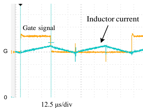
Figure 12. Input current (2 A/div) and gate signal (5 V/div) waveforms
