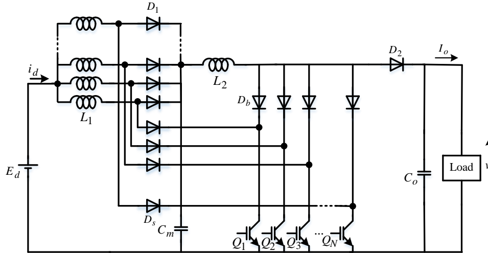
Figure 6. Second simplified cascade multiphase DC-DC boost converter
