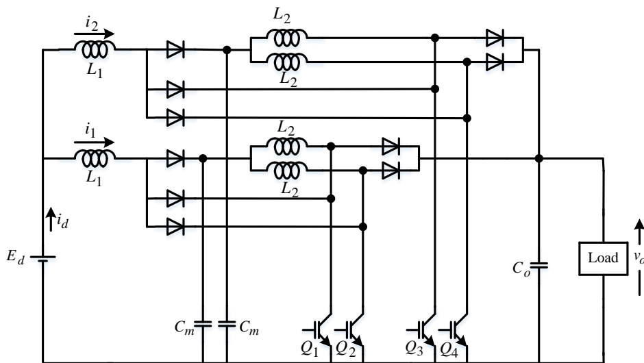
Figure 8. Simplified cascade four-phase DC-DC boost converter
