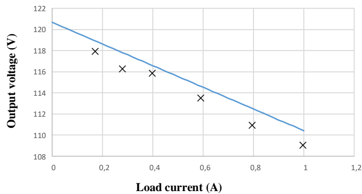
Figure 15. Output voltage as a function of load current
