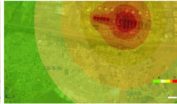
Figure 7. Noise mapping generated by the GNL1 and GNL2 complexes under meteorological conditions ( T = 25\text{ }^{\circ}\text{C} )
