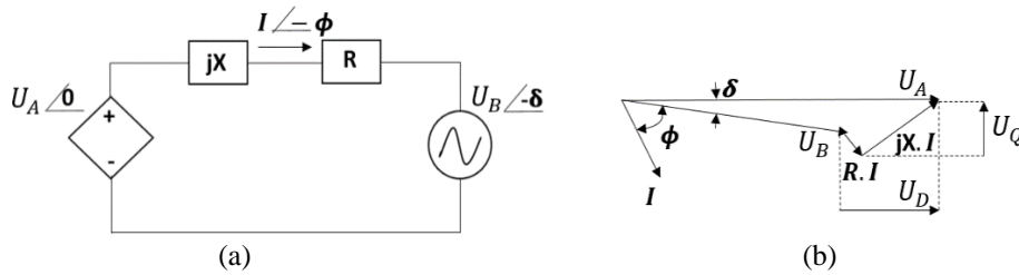
Figure 6. Modelling of power converter connected to the distribution network. (a) Equivalent circuit (b) phasor diagram
