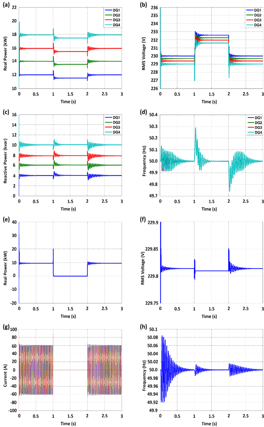
Figure 8. Microgrid and grid performance during intentional islanding scenario
