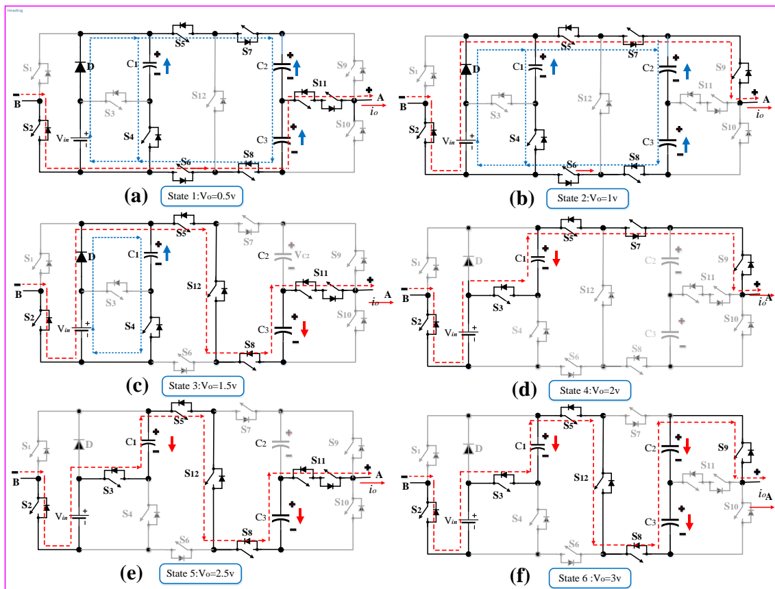
Figure 3. Operating modes of inverter during the positive half cycle
