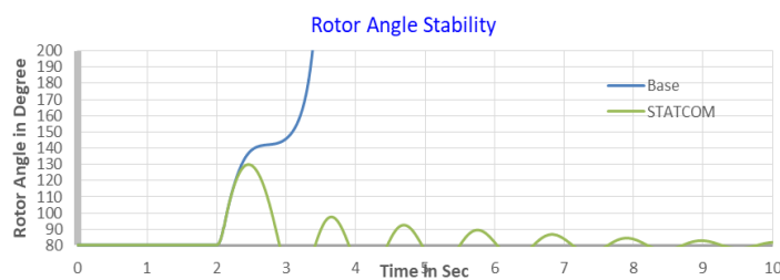
Figure 10. Plot of rotor angle stability of synchronous generators–1 for base case vs STATCOM
