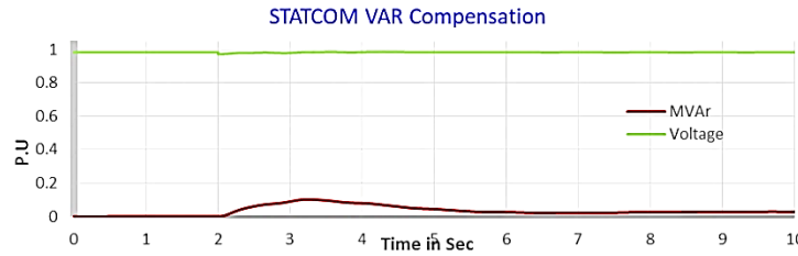
Figure 5. Plot of STATCOM dynamic VAR compensation
