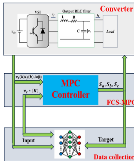
Figure 4. Block of the ANN-MPC's offline training procedure
