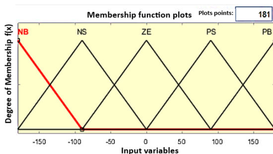
Figure 2. Membership function of fuzzy error and delta error
