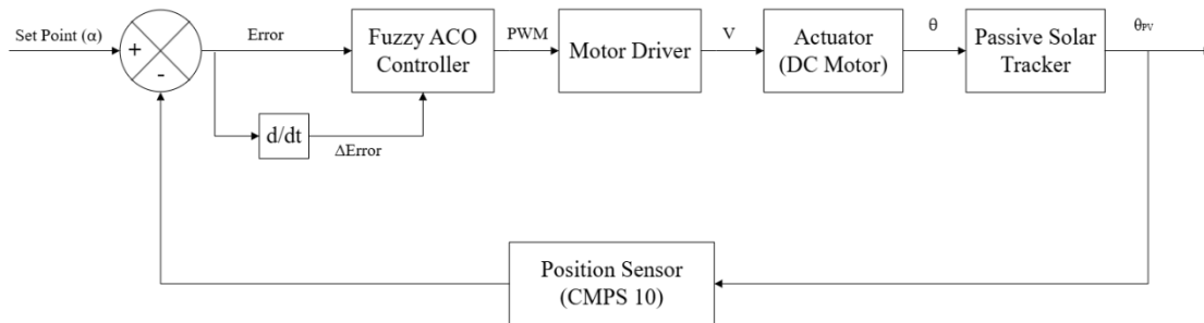
Figure 1. Block diagram of the solar tracker system
