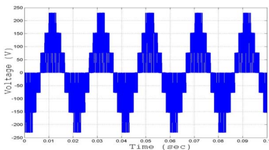
Figure 5. Multilevel Inverter Output Voltage with NFC
