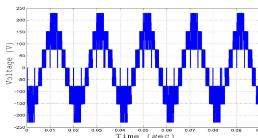
Figure 7. Multilevel Inverter Output Voltage with Proposed Technique
