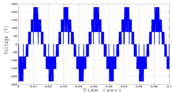
Figure 6. Multilevel Inverter Output Voltage with ANFIS
