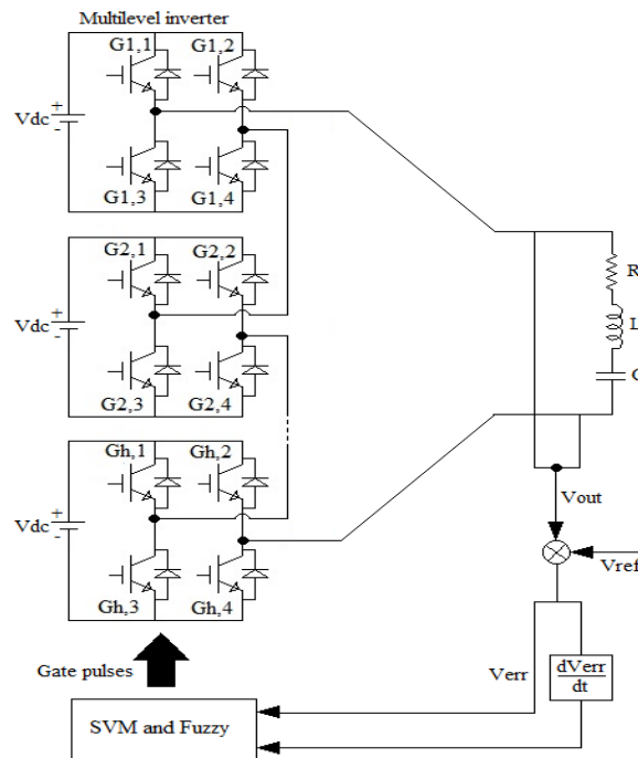
Figure 1. Structure of the Proposed Method
