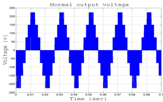
Figure 3. Seven Level Inverter Output Voltage without Controller
