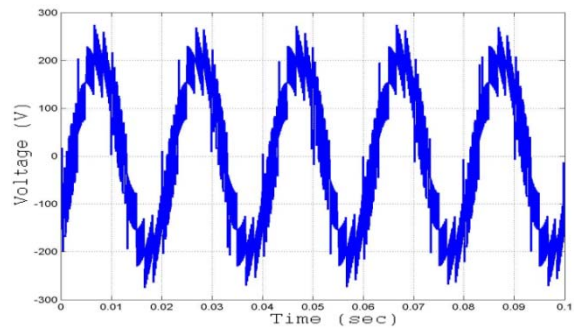
Figure 4. Difference between Normal Output and Reference Voltage
