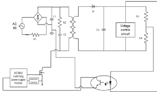
Figure 1. Circuit diagram of current mode controlled flyback converter
