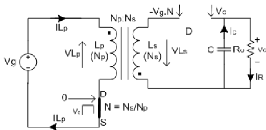
Figure 2. Mode 1; when Switch on
