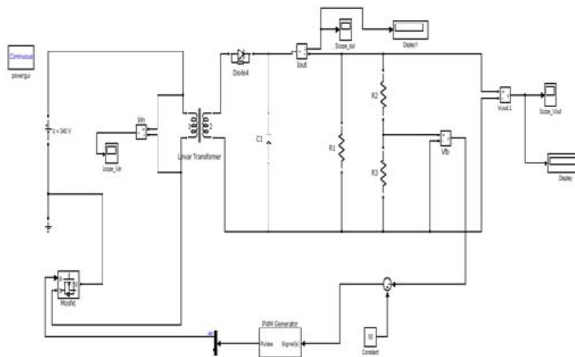
Figure 6. Matlab circuit for flyback converter
