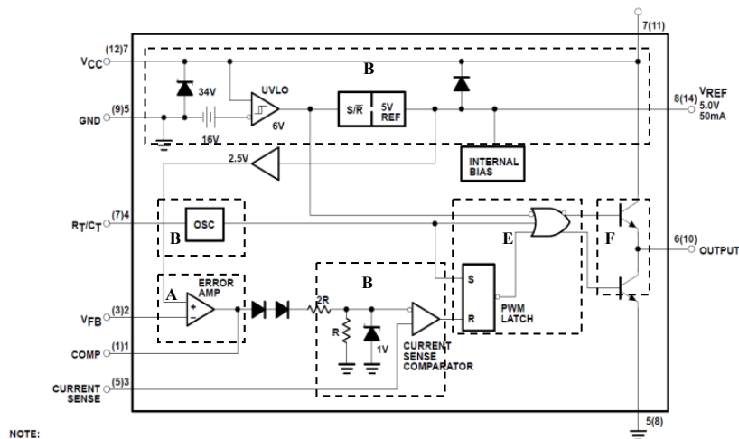
Figure 4. UC3842 block diagram
