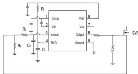
Figure 5. Control circuit
