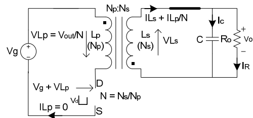
Figure 3. Mode 2; when Switch off
