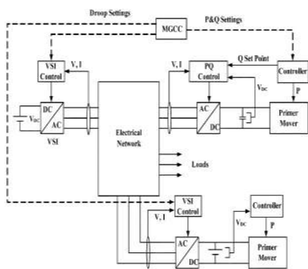
Figure 4. Control scheme for MMO
