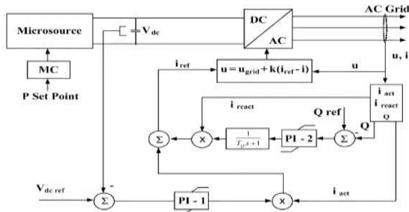
Figure 2. PQ inverter control system
