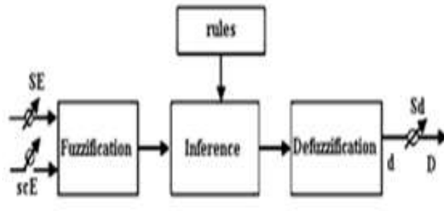
Figure 7. General diagram of fuzzy controller
