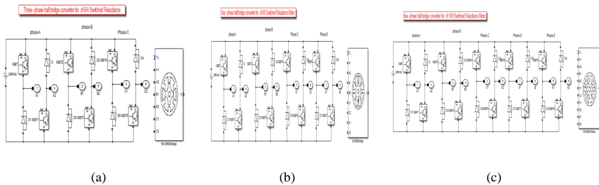
Figure 2. Bridge Converter for (a) 6/4 SRM, (b) 8/6 SRM, (c) 10/8 SRM
