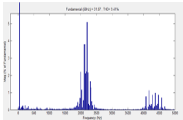
(b) THD of current of half bridge converter
