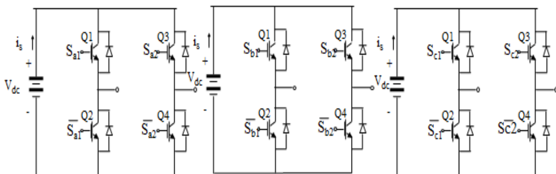
Figure 3. three-level inverter
