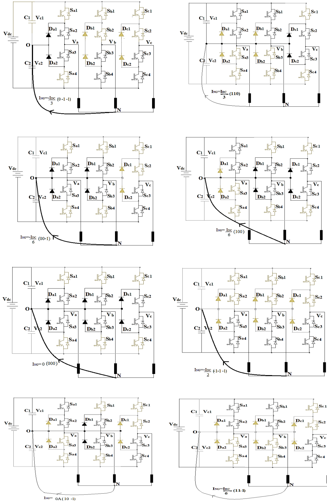
Figure 4. Different Switching states and its Circulating Current
