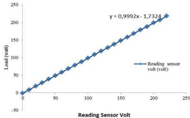
Figure 12. The graphic of calibration of ZMPT101B sensor from the proposed design
