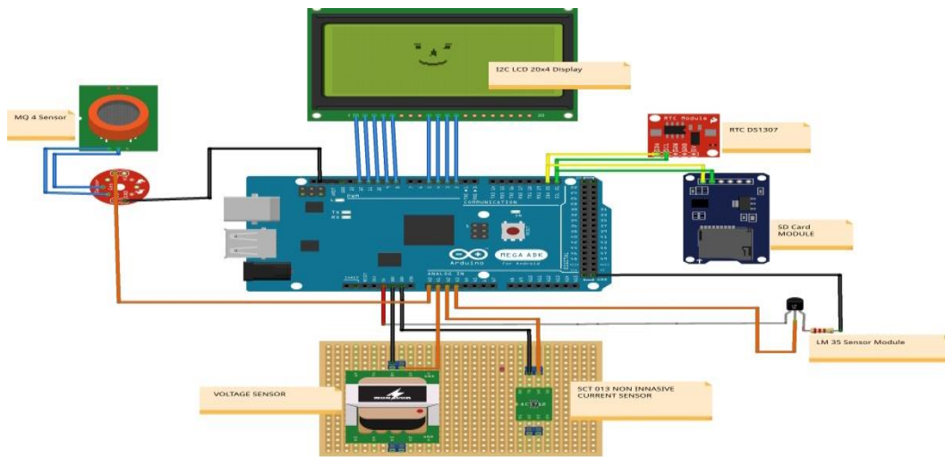
Figure 9. The schematic circuit of HPS LFG-PV-genset sensor
