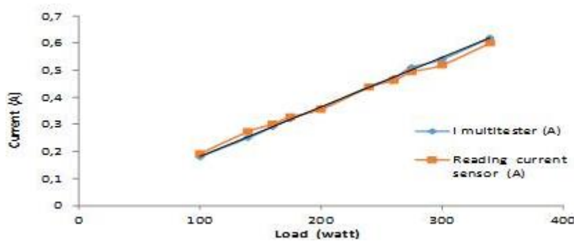
Figure 11. The graphic of calibration of SCT 013 non-invasive sensor from the proposed design
