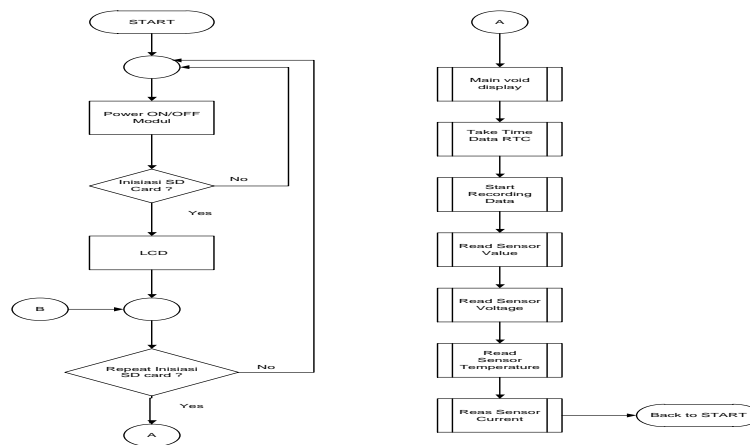
Figure 8. Flowchart of the processes of HPS LFG-PV-genset calibration measurement
