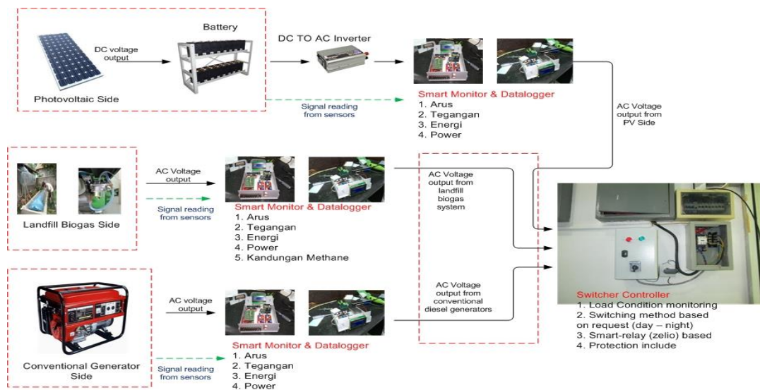
Figure 1. The schematic sequence of the system
