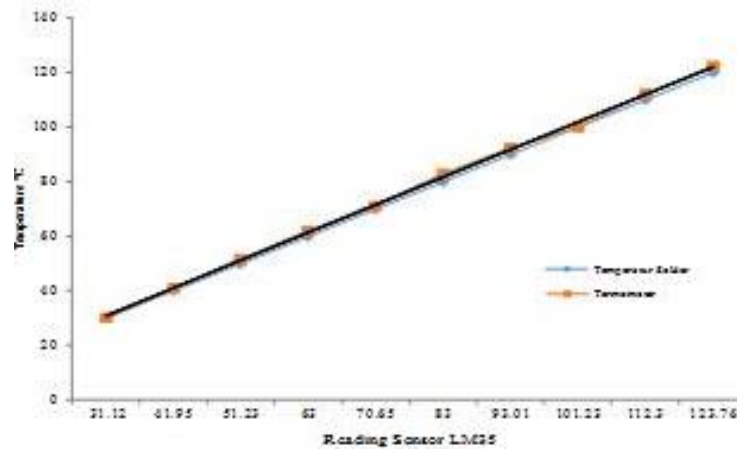
Figure 10. The graphic of calibration of MQ sensor resulted from the proposed design
