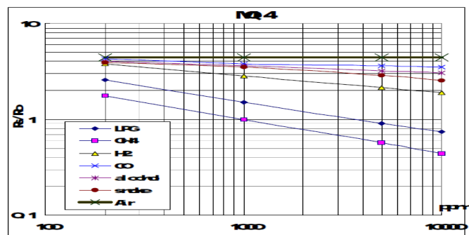
Figure 3. Characteristics of MQ4 sensor
